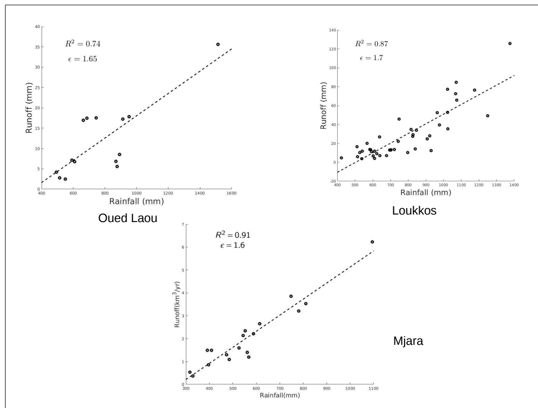
Figure 10. Elasticity coefficient estimation for the three watersheds with regression method
